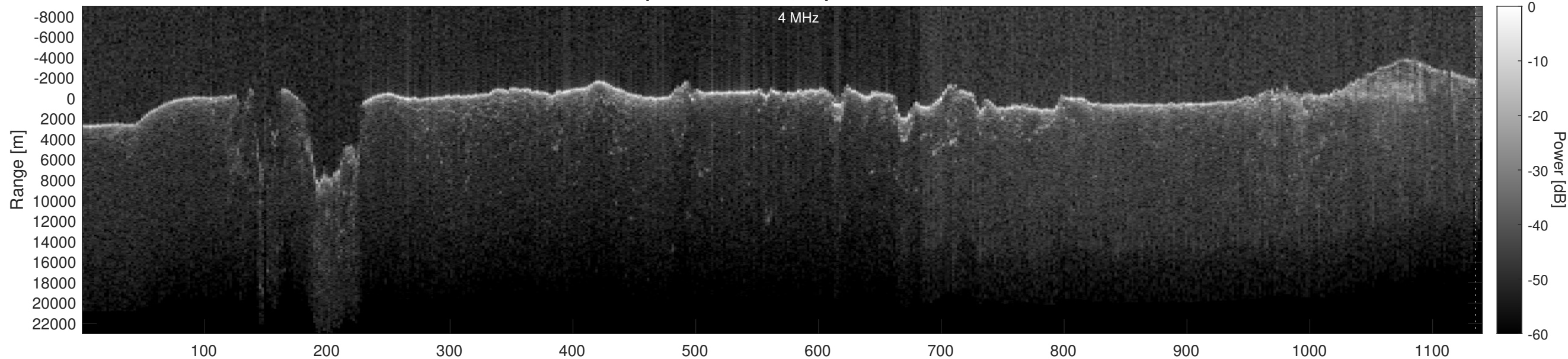
Orbit 21584, Optimized, Window, Depth-Corrected, Channel 2
