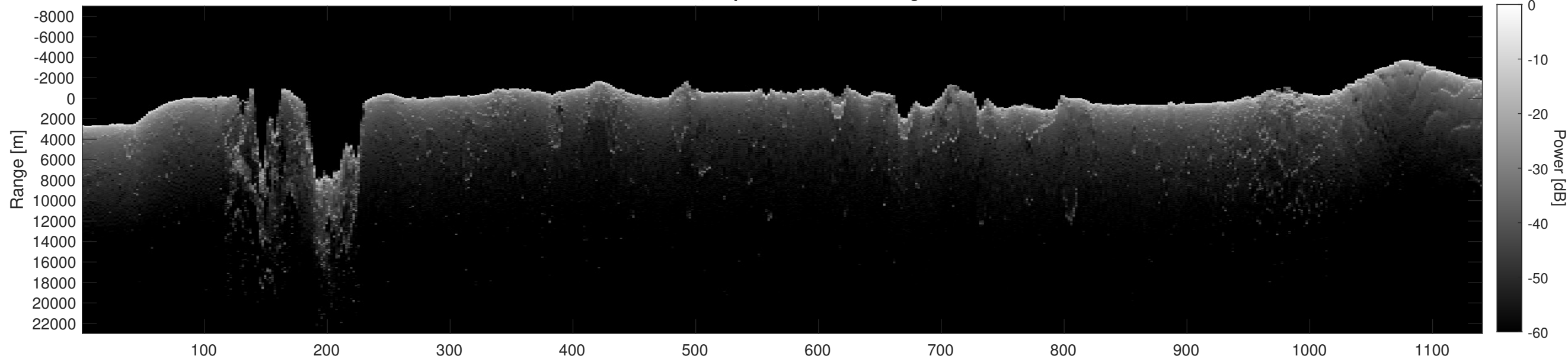
Orbit 21584, Depth-Corrected Cluttergram
