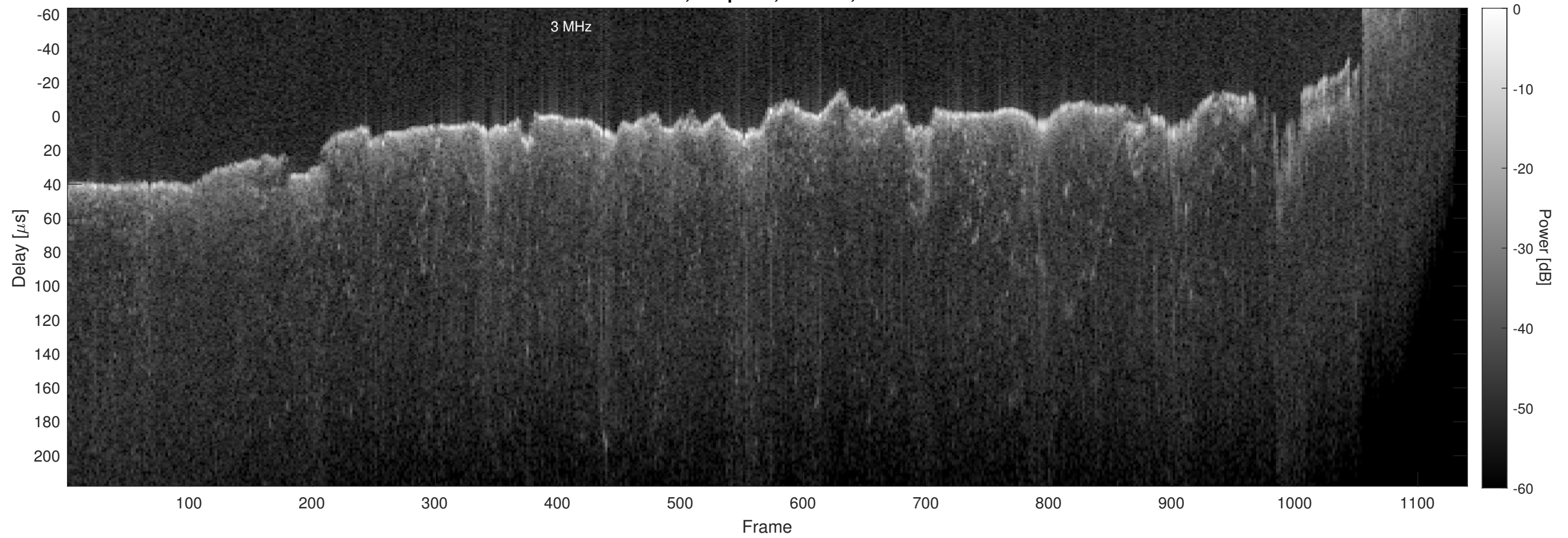
Orbit 21585, Chapman, Window, Channel 2
