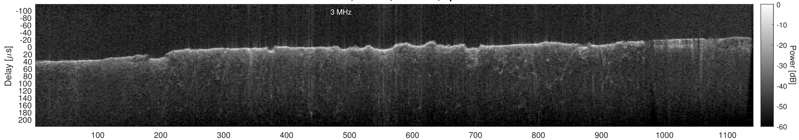
Orbit 21585, Cluttergram
