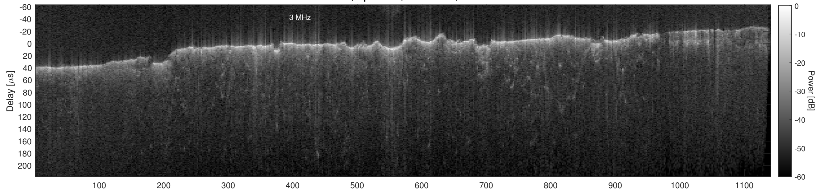
Orbit 21585, Cluttergram
