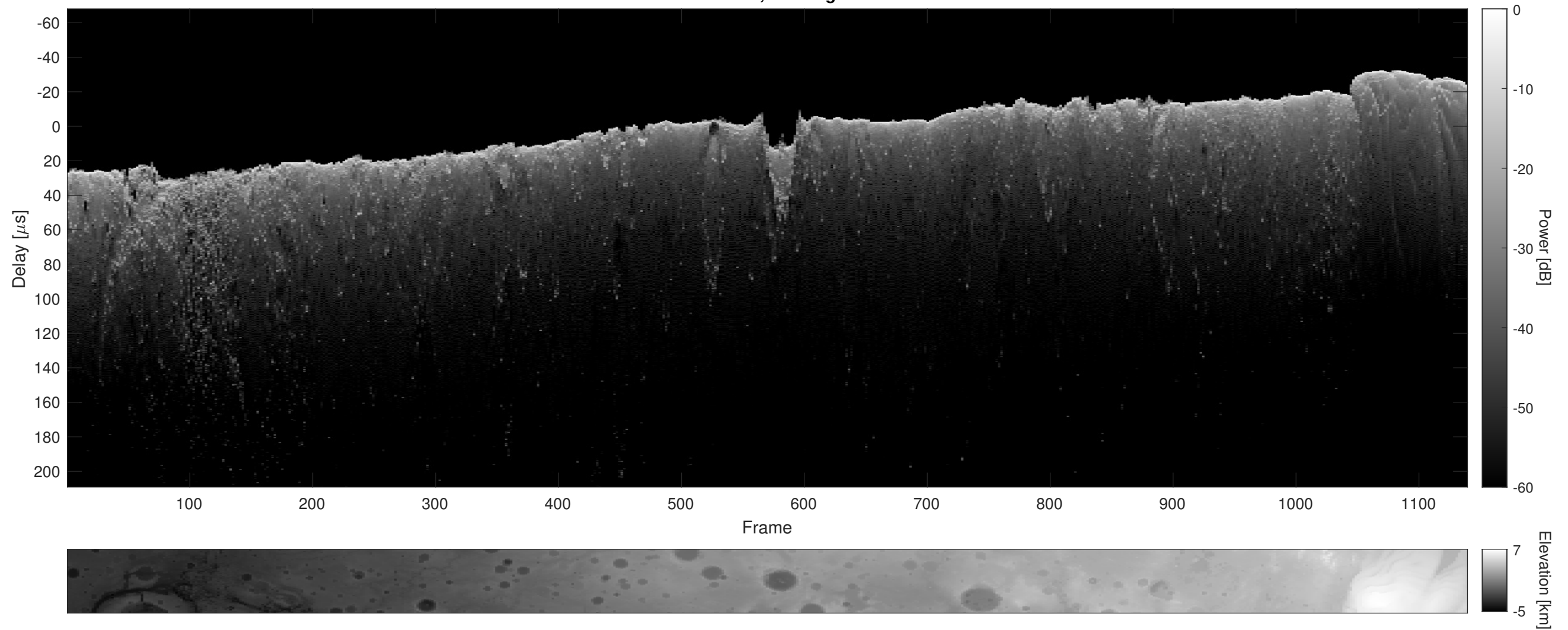
Orbit 21587, Cluttergram
