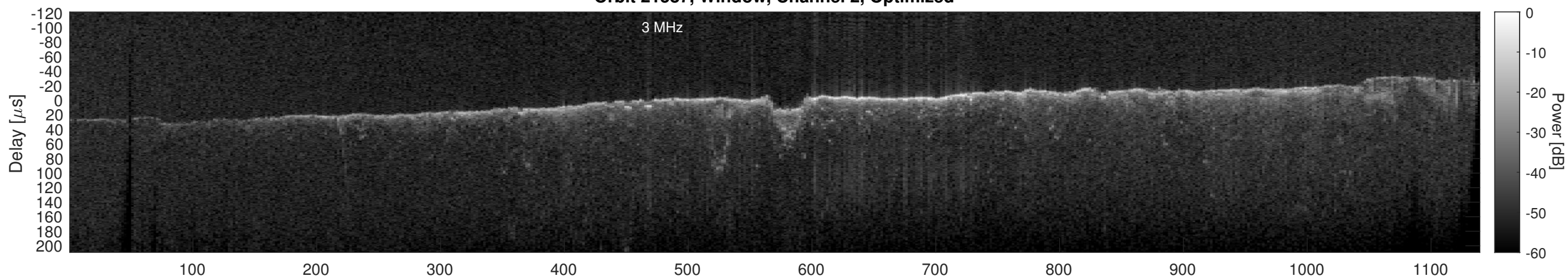
Orbit 21587, Cluttergram
