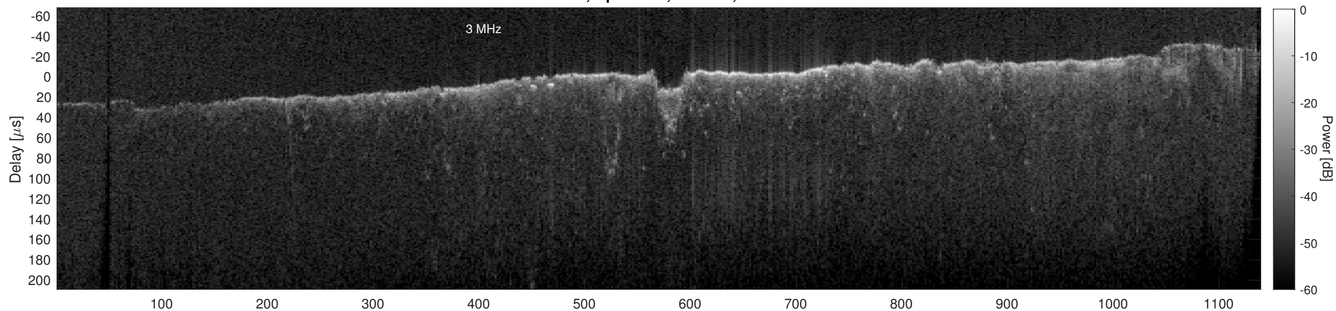
Orbit 21587, Cluttergram
