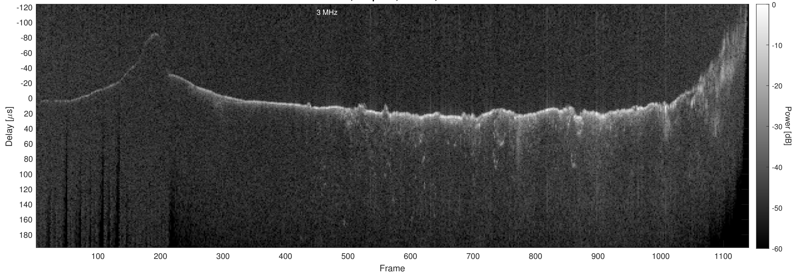
Orbit 21588, Chapman, Window, Channel 2
