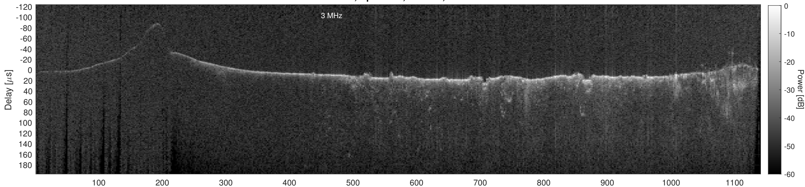
Orbit 21588, Cluttergram
