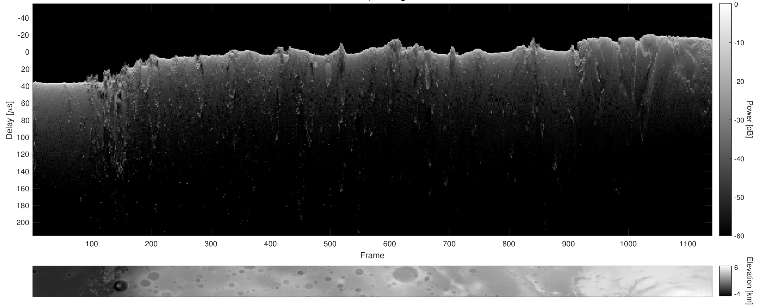
Orbit 21589, Cluttergram
