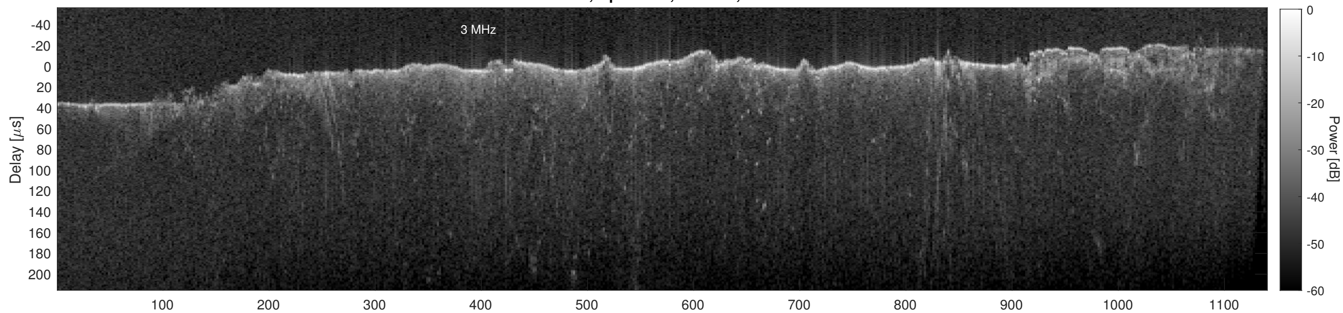
Orbit 21589, Cluttergram
