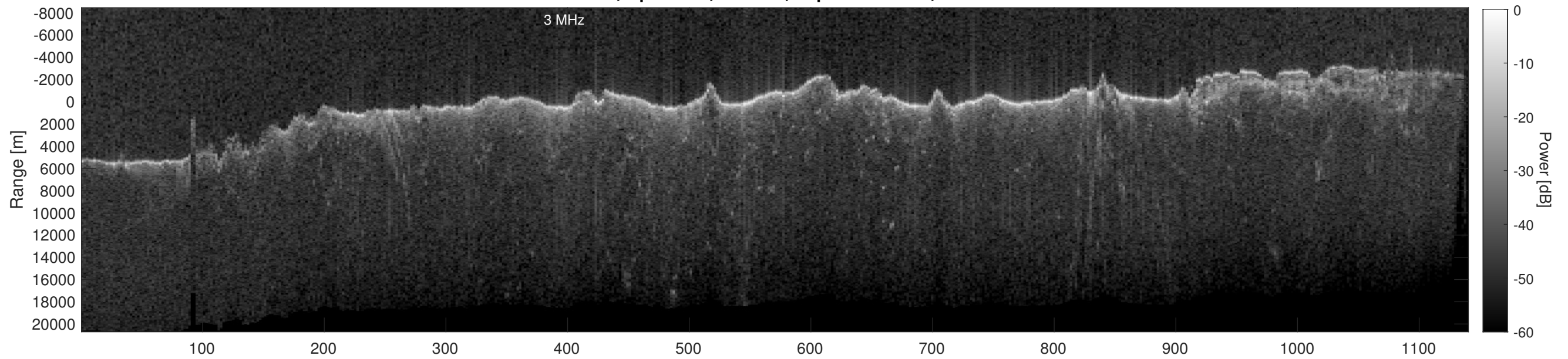
Orbit 21589, Depth-Corrected Cluttergram
