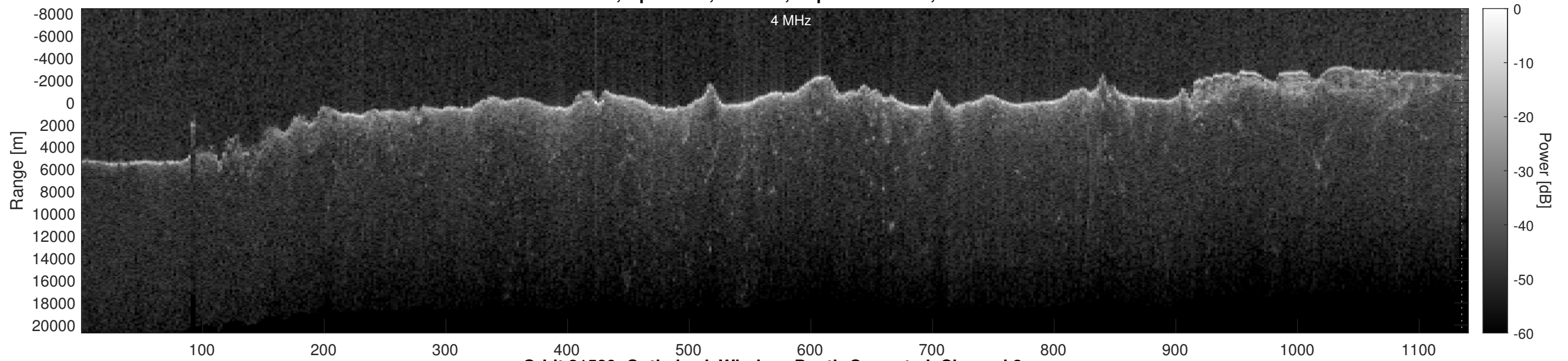
Orbit 21589, Optimized, Window, Depth-Corrected, Channel 2
