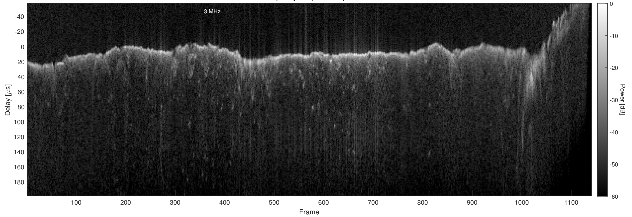
Orbit 21590, Chapman, Window, Channel 2
