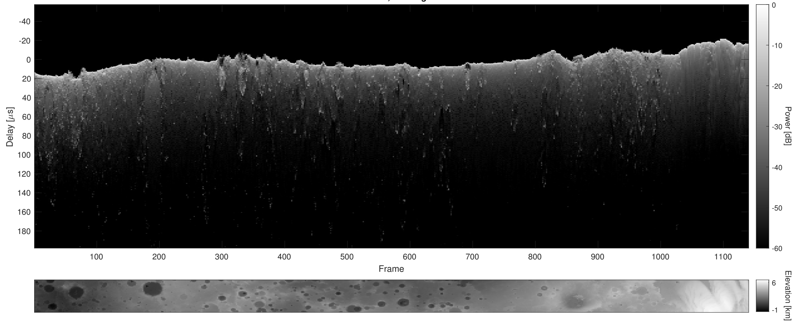
Orbit 21590, Cluttergram
