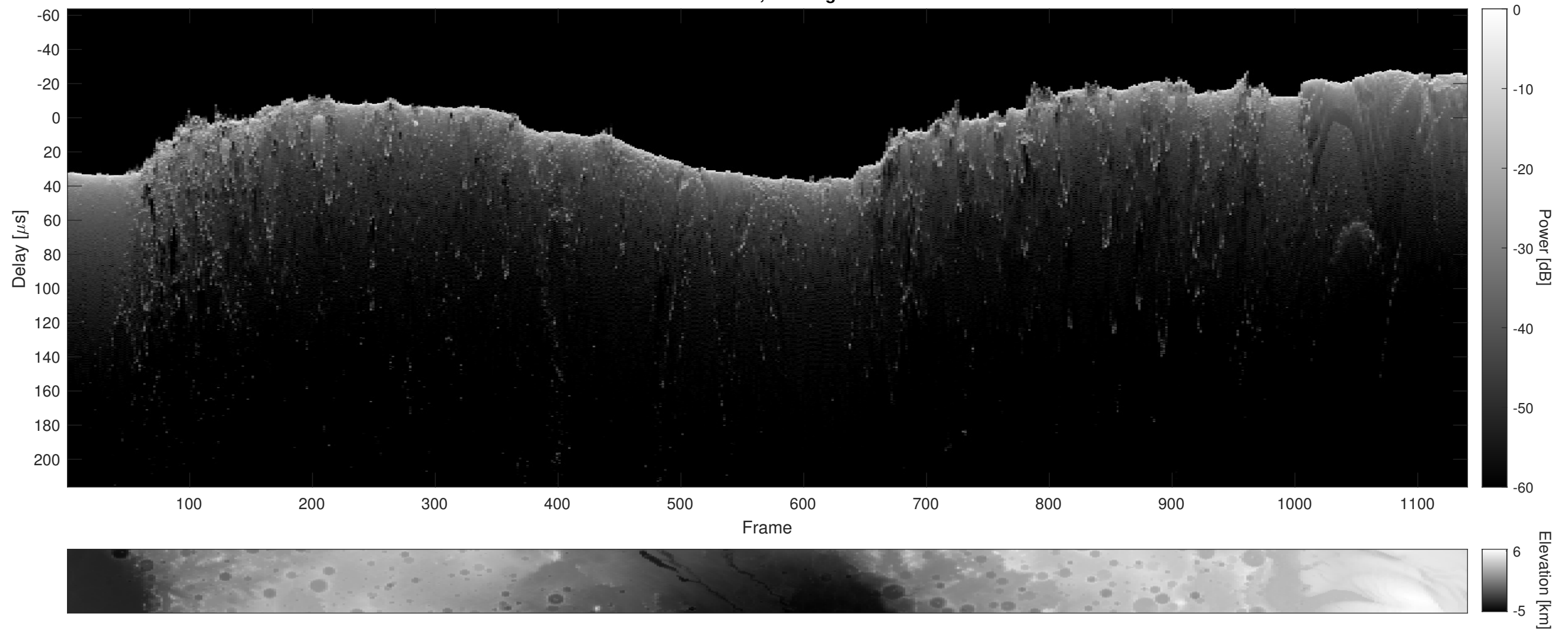
Orbit 21593, Cluttergram
