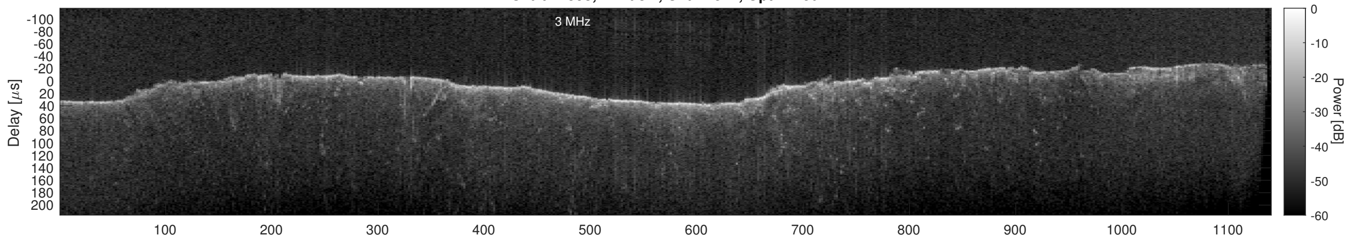
Orbit 21593, Cluttergram
