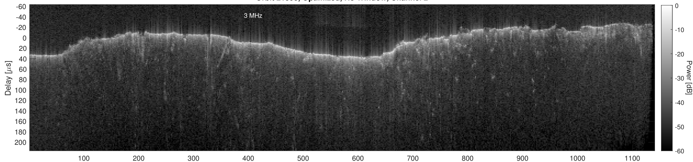
Orbit 21593, Cluttergram
