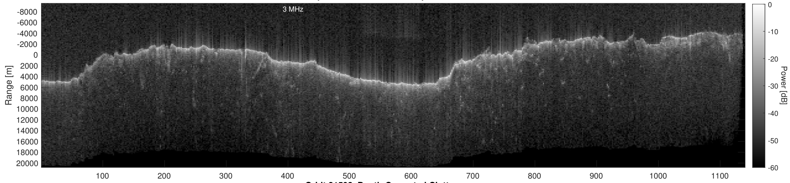
Orbit 21593, Depth-Corrected Cluttergram
