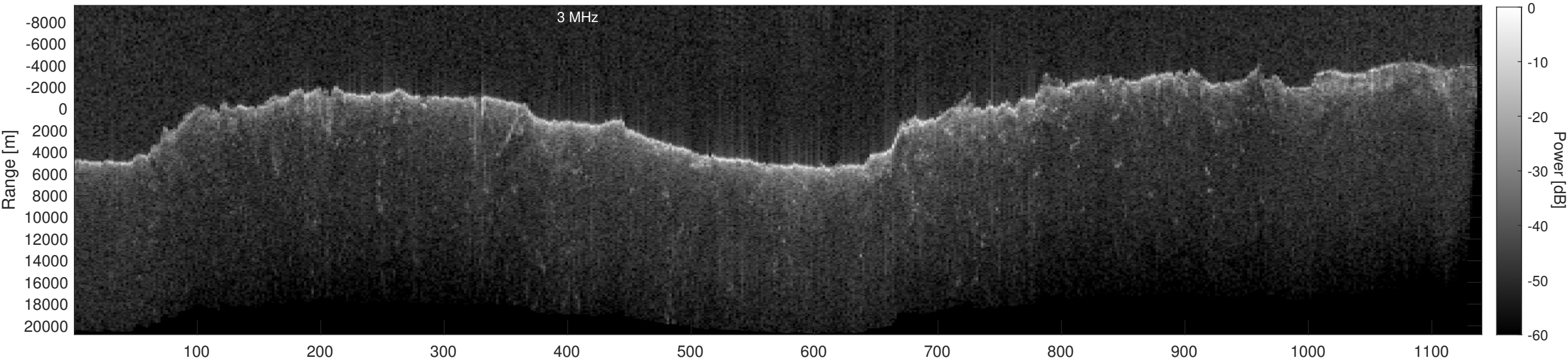
Orbit 21593, Depth-Corrected Cluttergram
