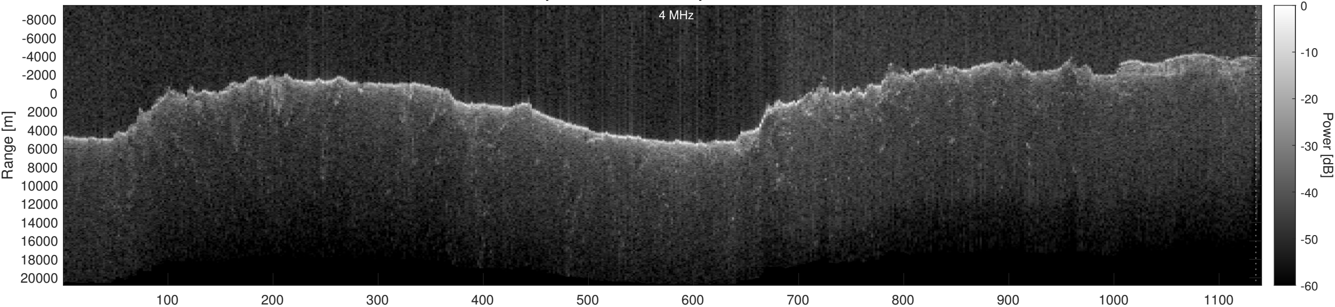
Orbit 21593, Optimized, Window, Depth-Corrected, Channel 2
