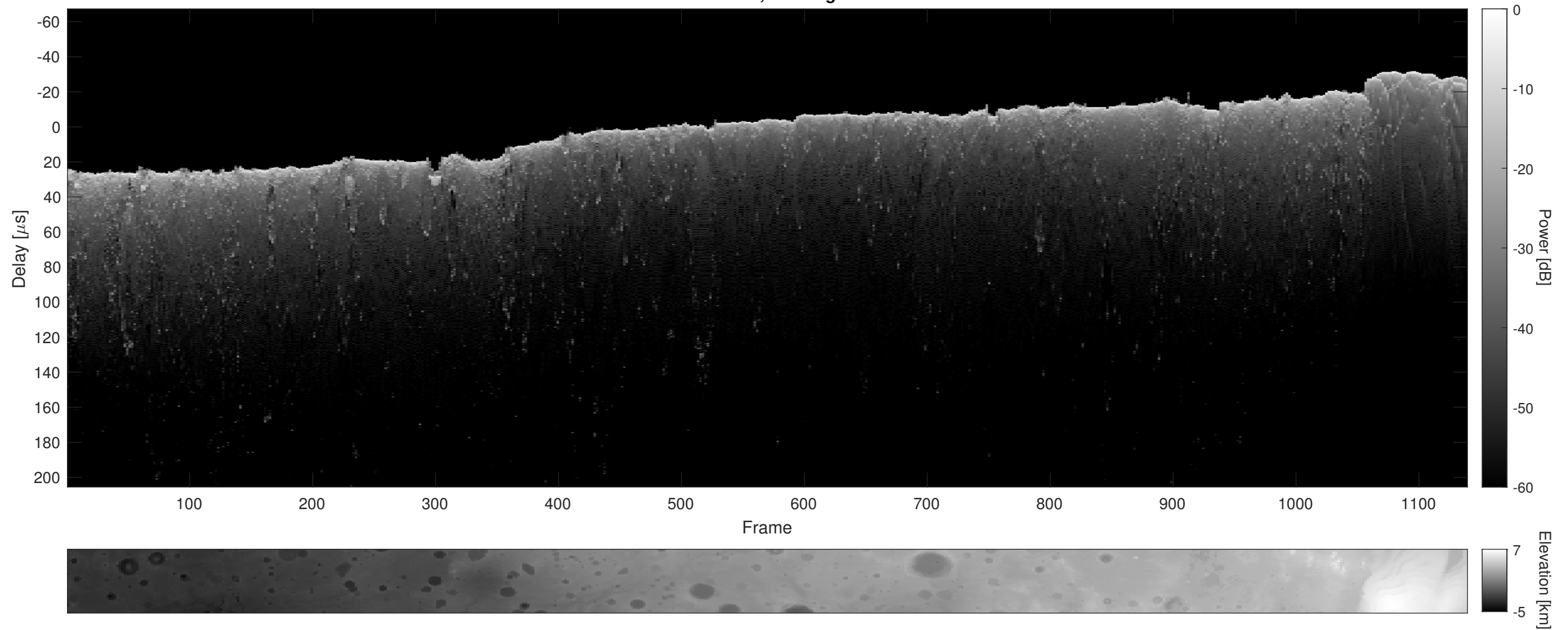
Orbit 21594, Cluttergram
