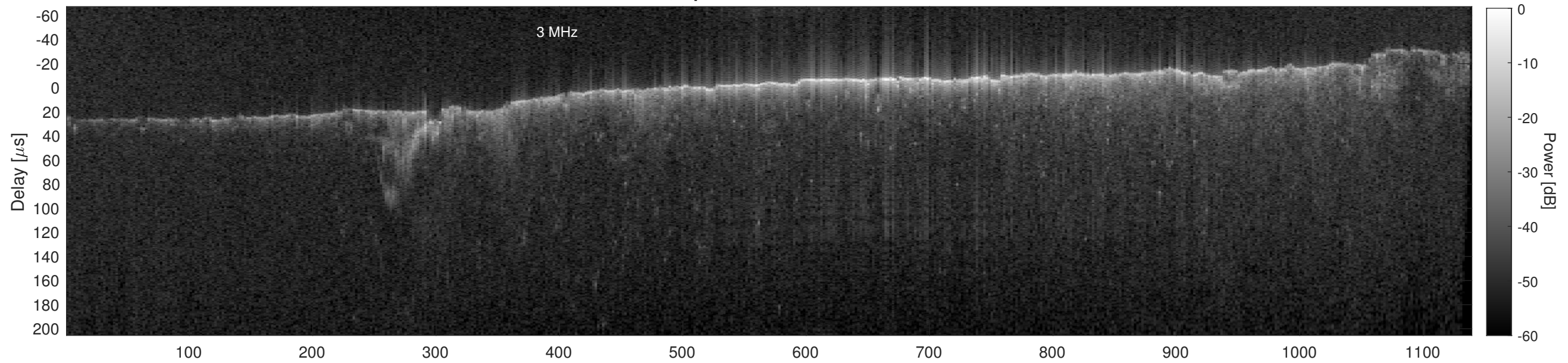
Orbit 21594, Cluttergram
