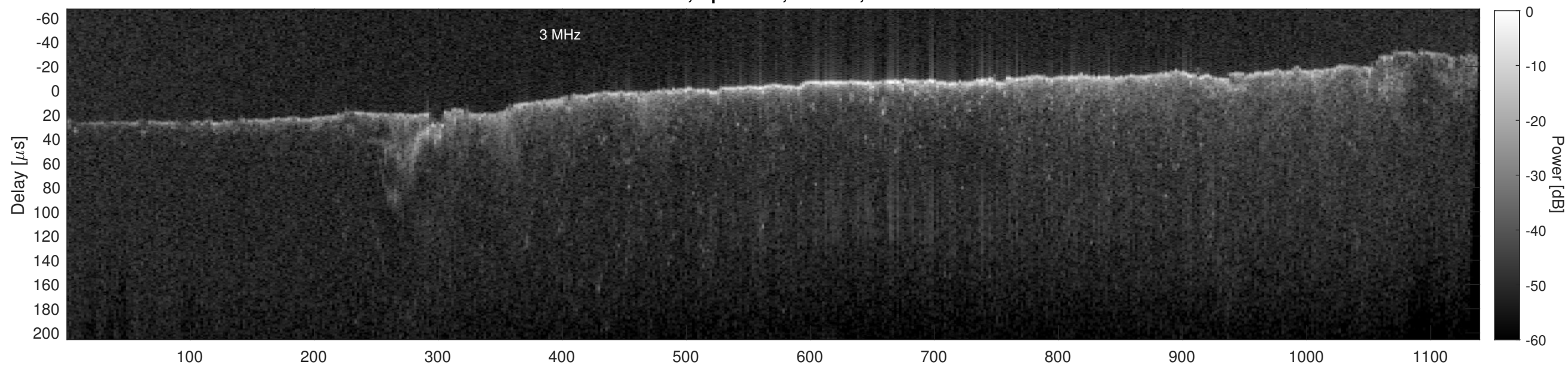
Orbit 21594, Cluttergram
