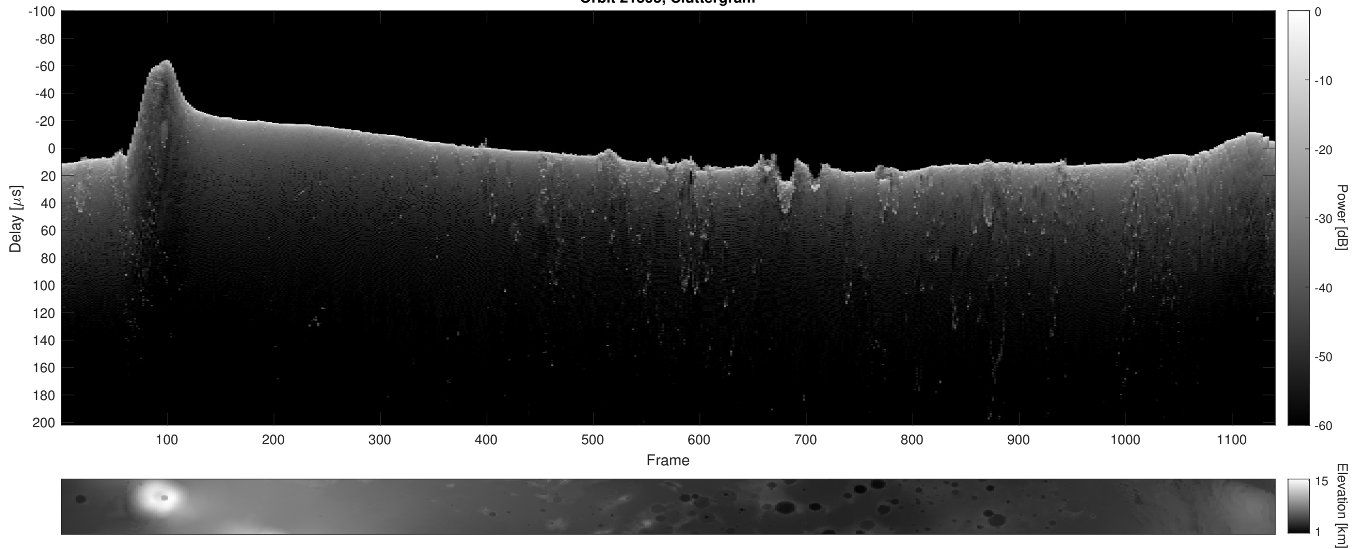
Orbit 21595, Cluttergram
