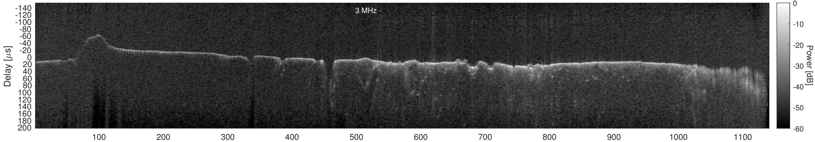
Orbit 21595, Window, Channel 2, Chapman
