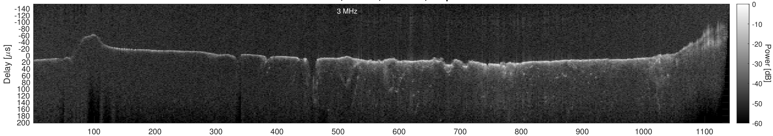
Orbit 21595, Window, Channel 2, Optimized
