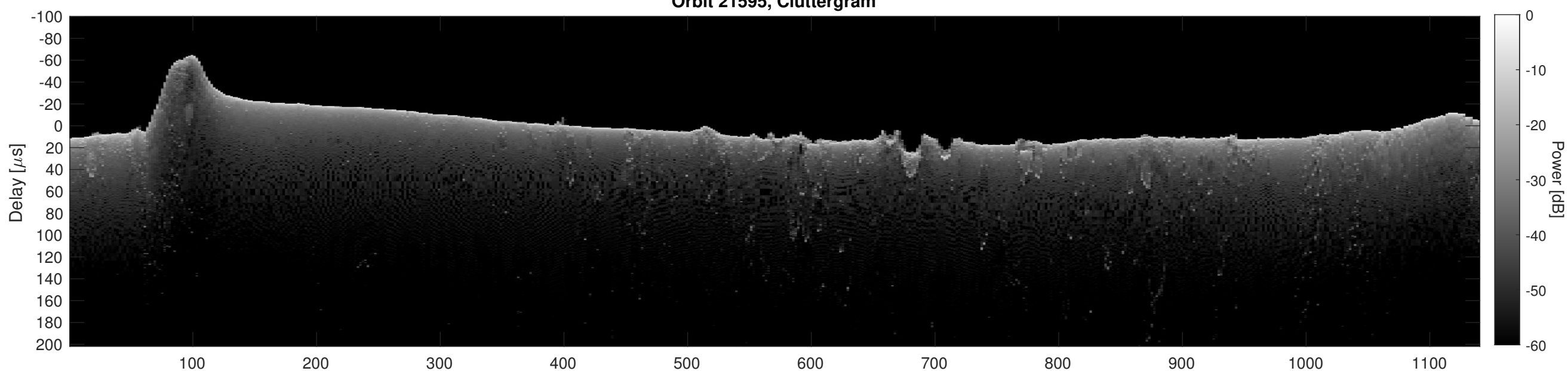
Orbit 21595, Cluttergram
