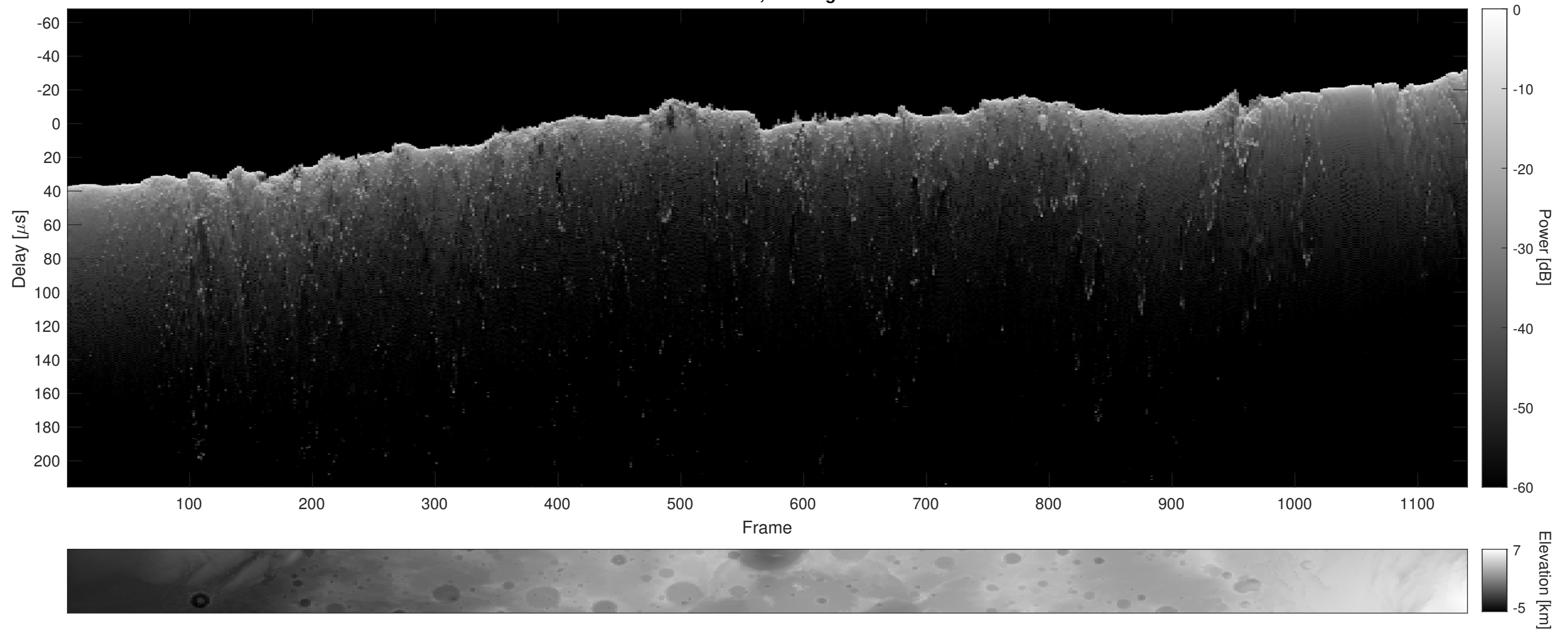
Orbit 21599, Cluttergram
