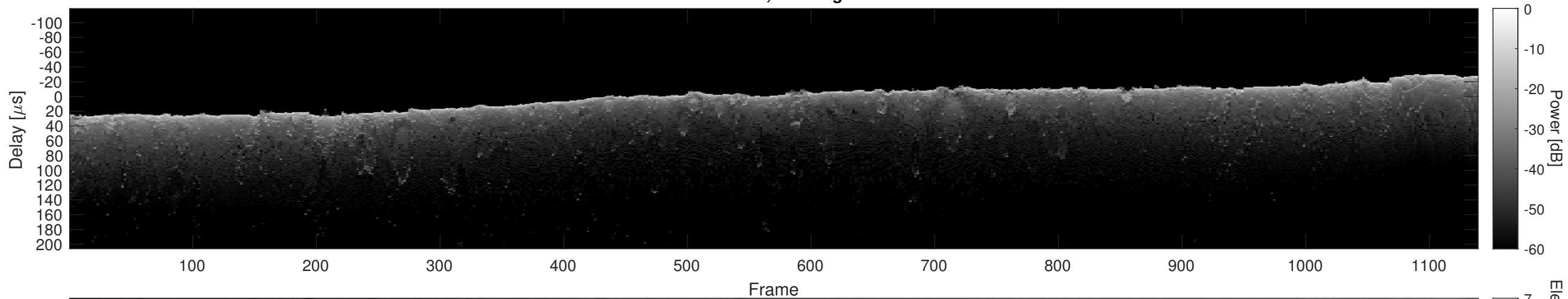
Orbit 21601, Cluttergram
