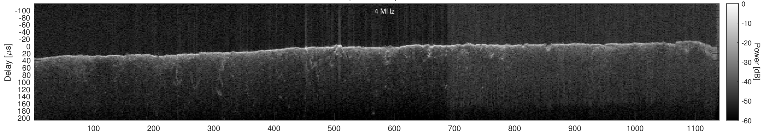
Orbit 21601, Window, Channel 1, Chapman
