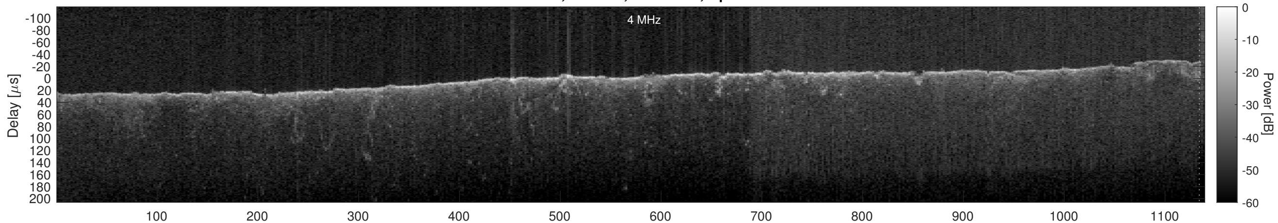
Orbit 21601, Cluttergram
