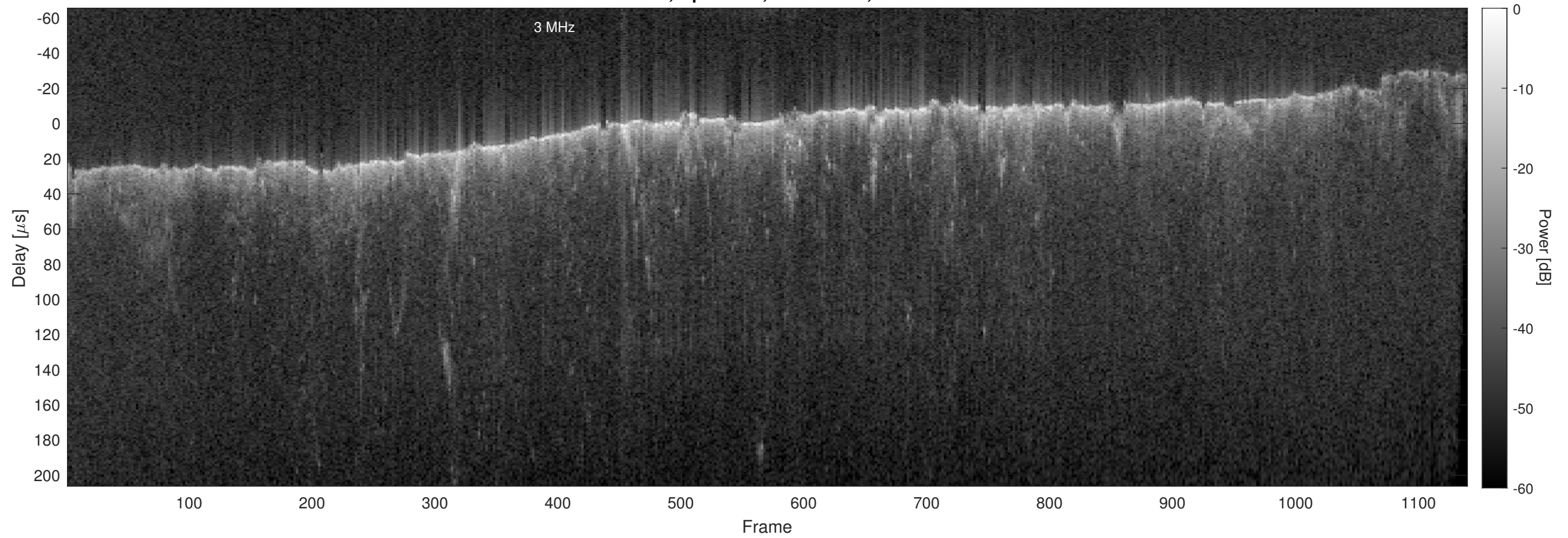
Orbit 21601, Optimized, No Window, Channel 2
