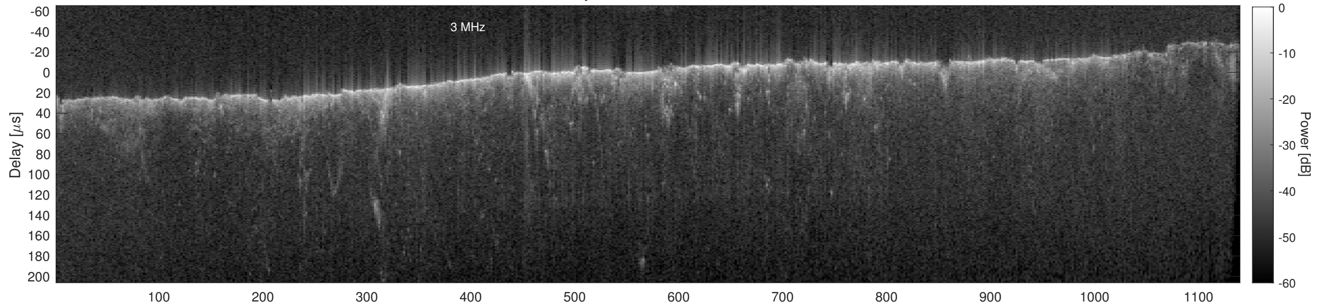
Orbit 21601, Cluttergram
