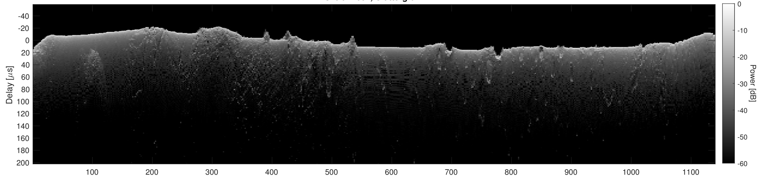
Orbit 21602, Cluttergram
