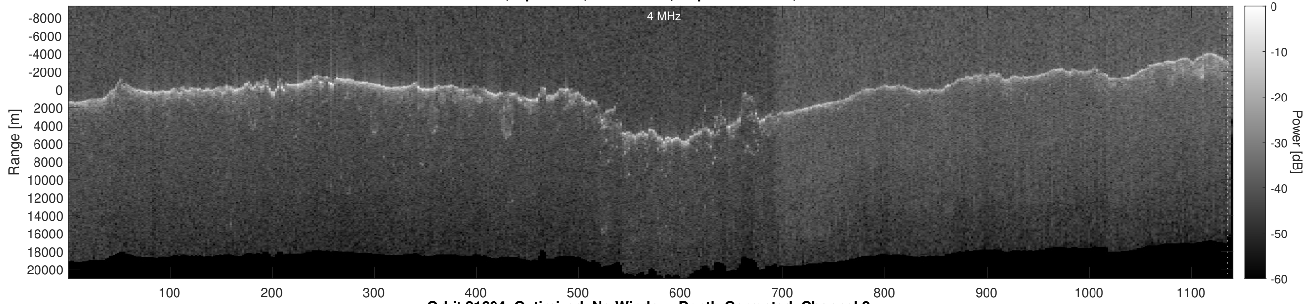
Orbit 21604, Optimized, No Window, Depth-Corrected, Channel 2
