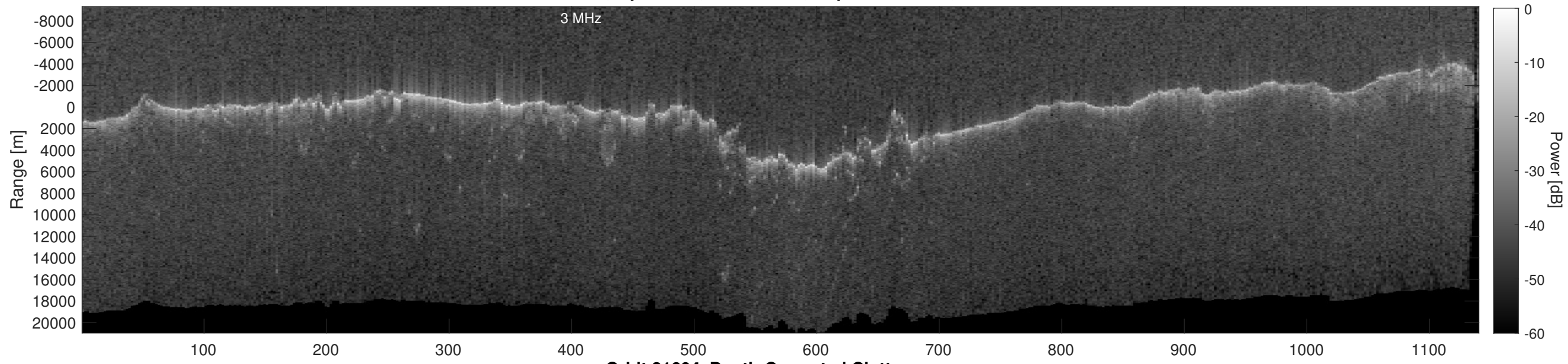
Orbit 21604, Depth-Corrected Cluttergram
