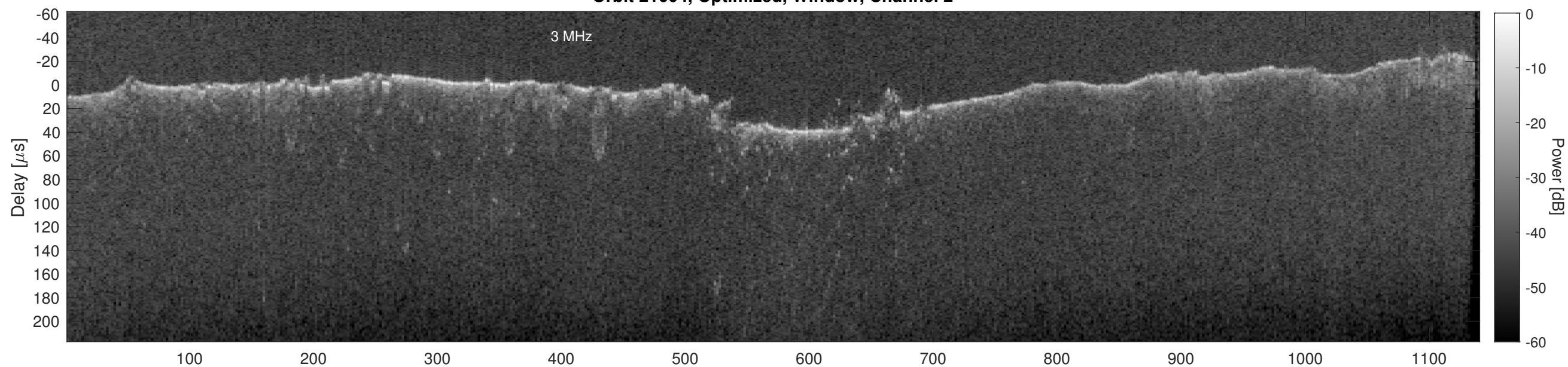
Orbit 21604, Cluttergram
