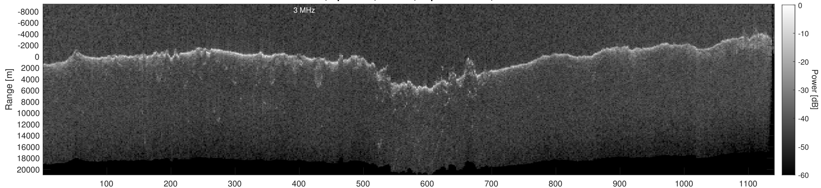
Orbit 21604, Depth-Corrected Cluttergram
