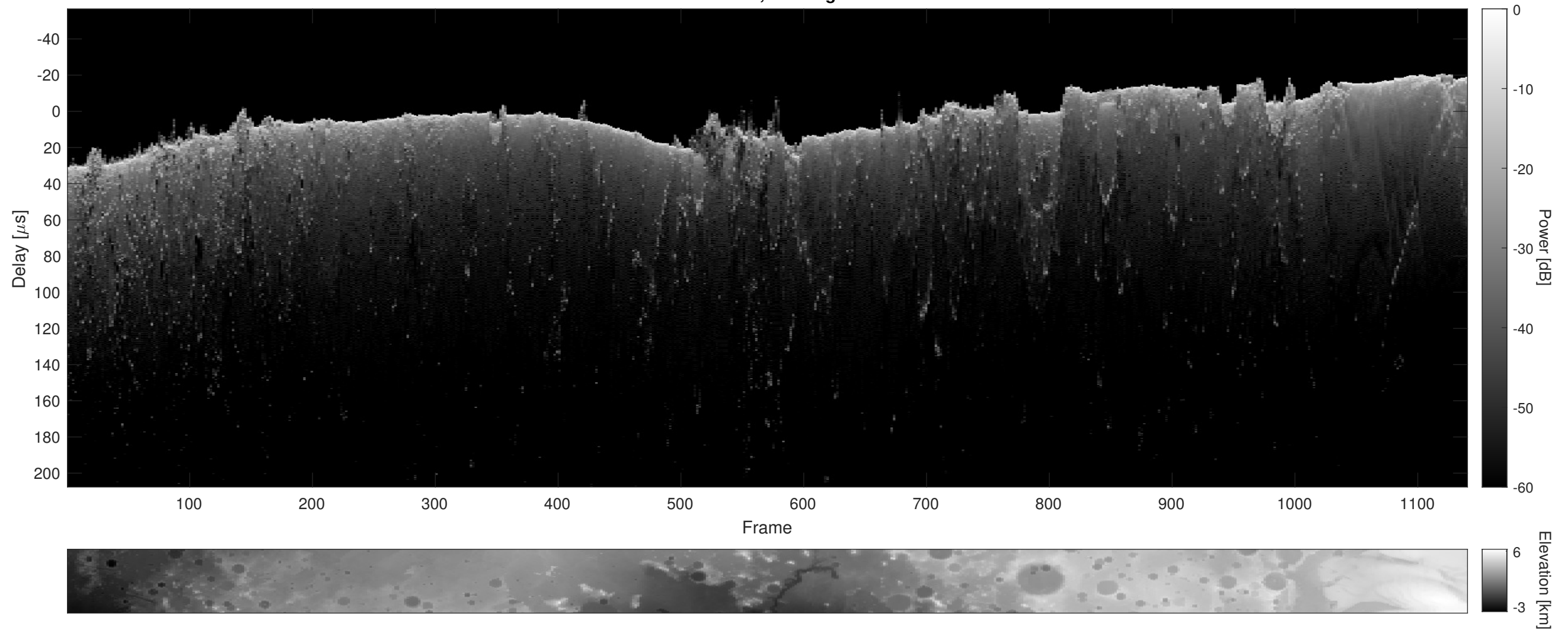
Orbit 21607, Cluttergram
