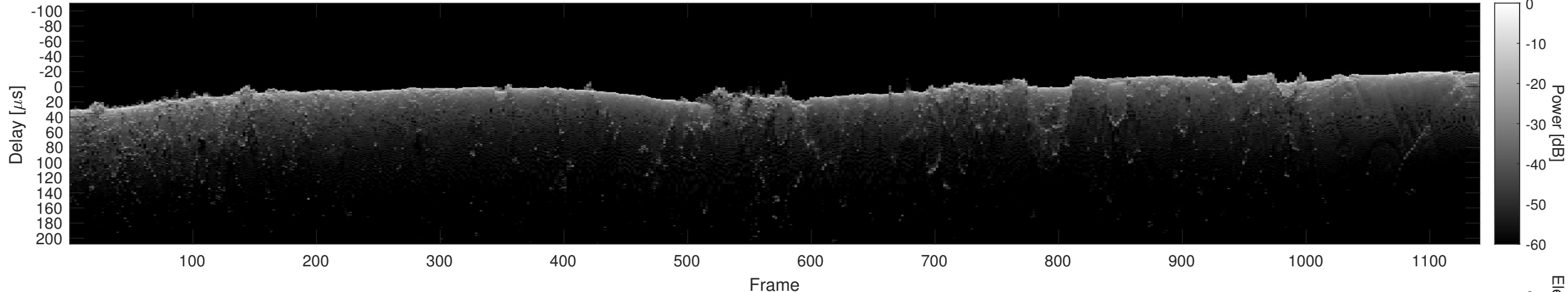
Orbit 21607, Cluttergram
