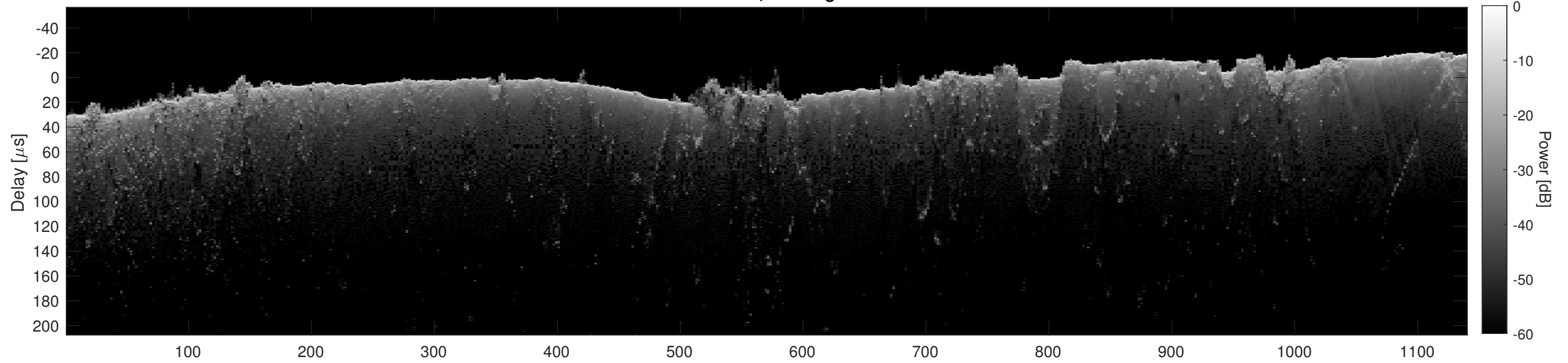
Orbit 21607, Cluttergram
