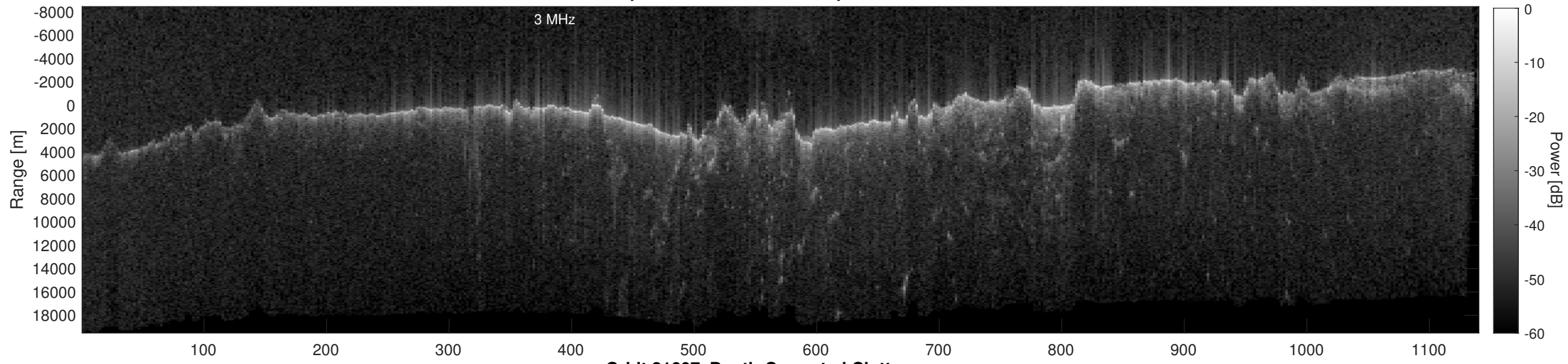
Orbit 21607, Depth-Corrected Cluttergram
