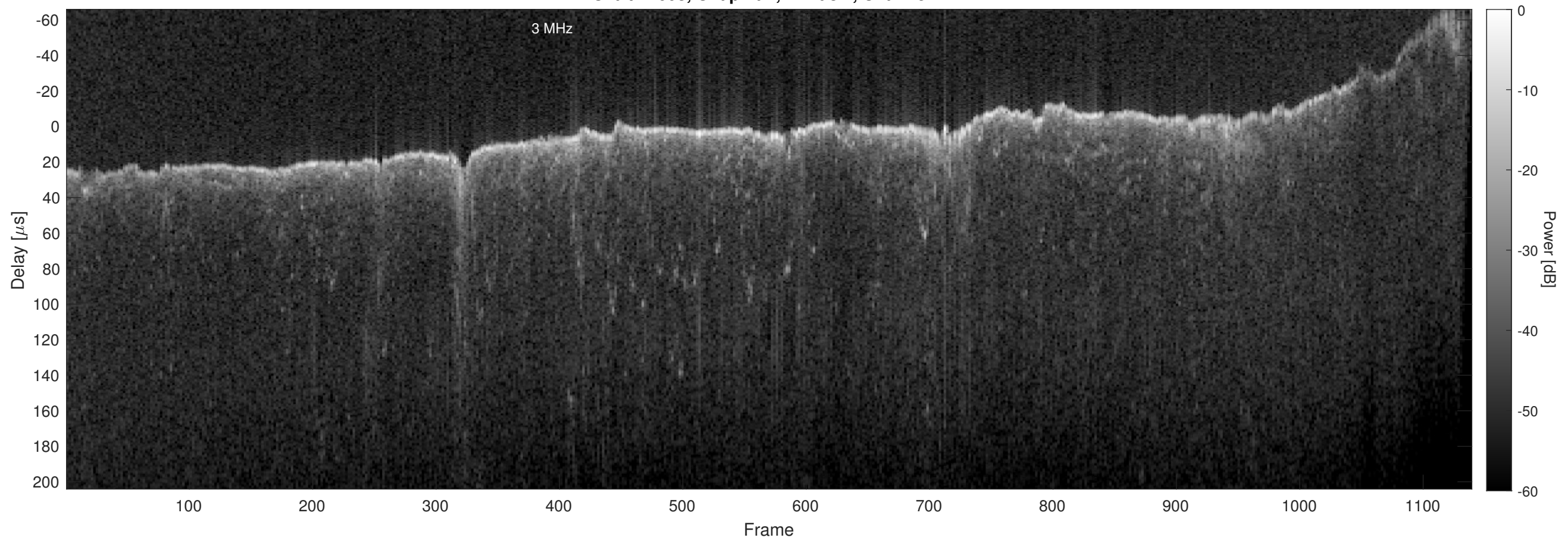
Orbit 21608, Chapman, Window, Channel 2
