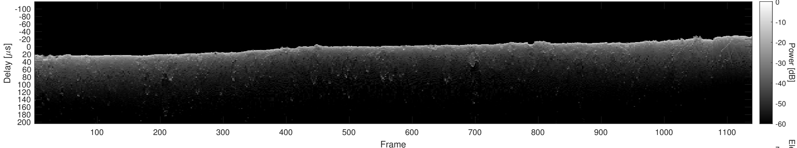
Orbit 21608, Cluttergram
