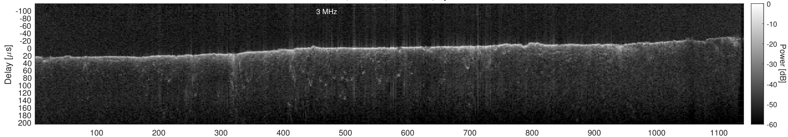
Orbit 21608, Cluttergram
