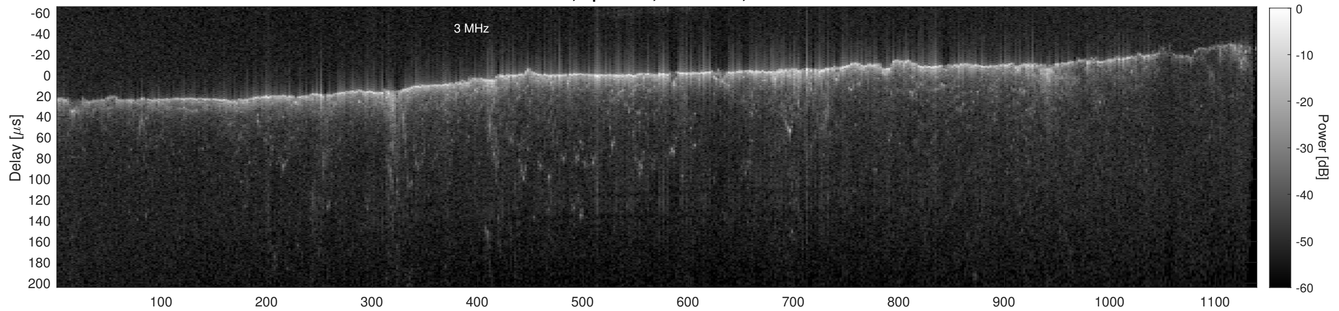
Orbit 21608, Cluttergram
