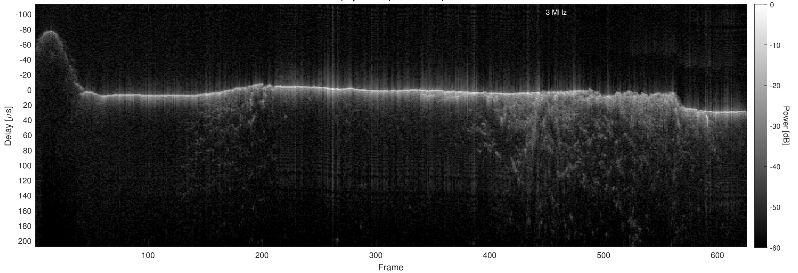
Orbit 21609, Optimized, No Window, Channel 2
