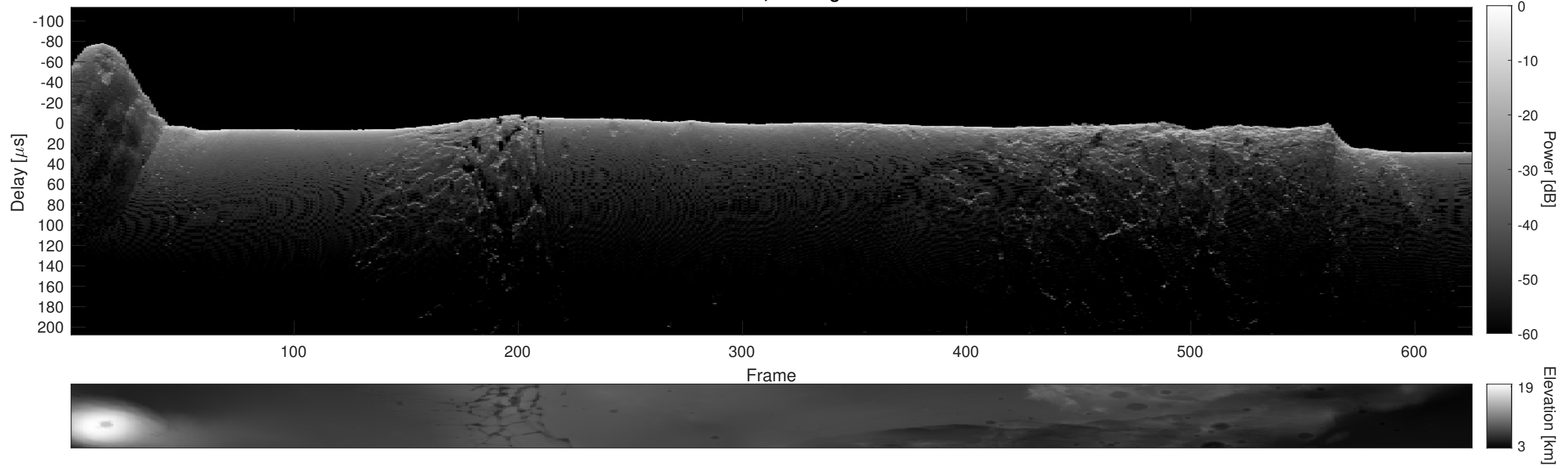
Orbit 21609, Cluttergram
