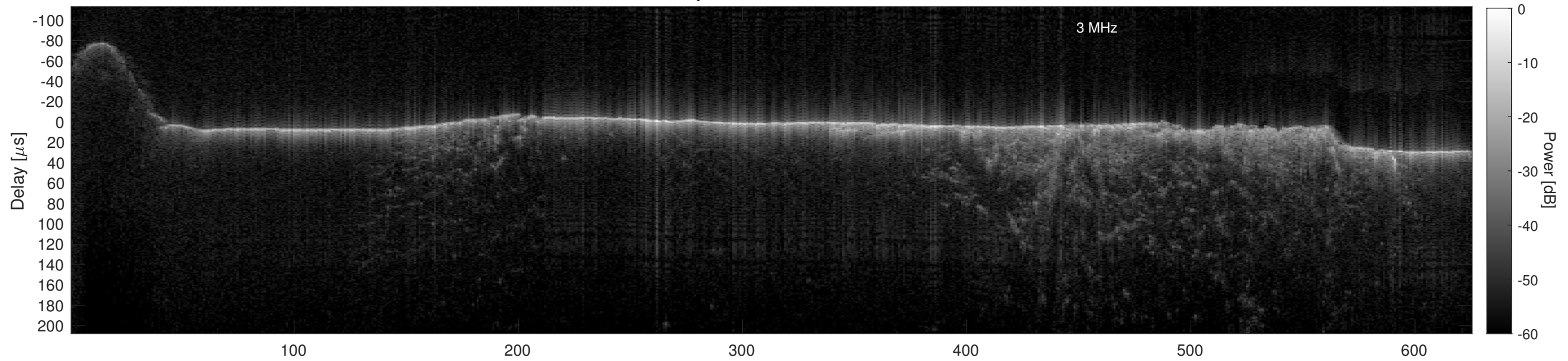
Orbit 21609, Cluttergram
