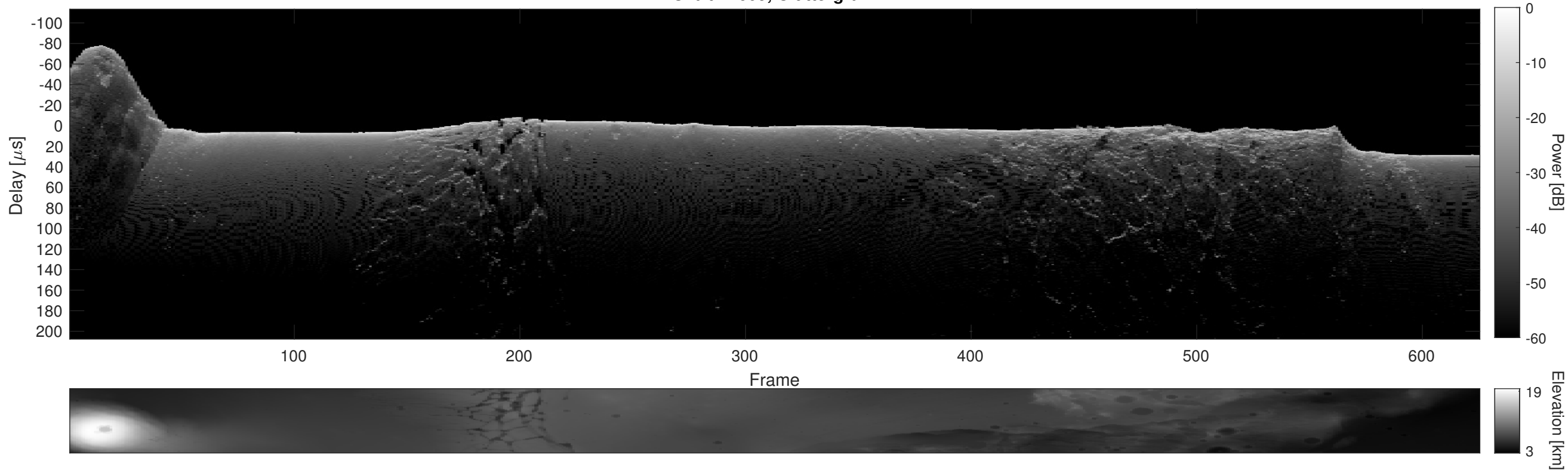
Orbit 21609, Cluttergram
