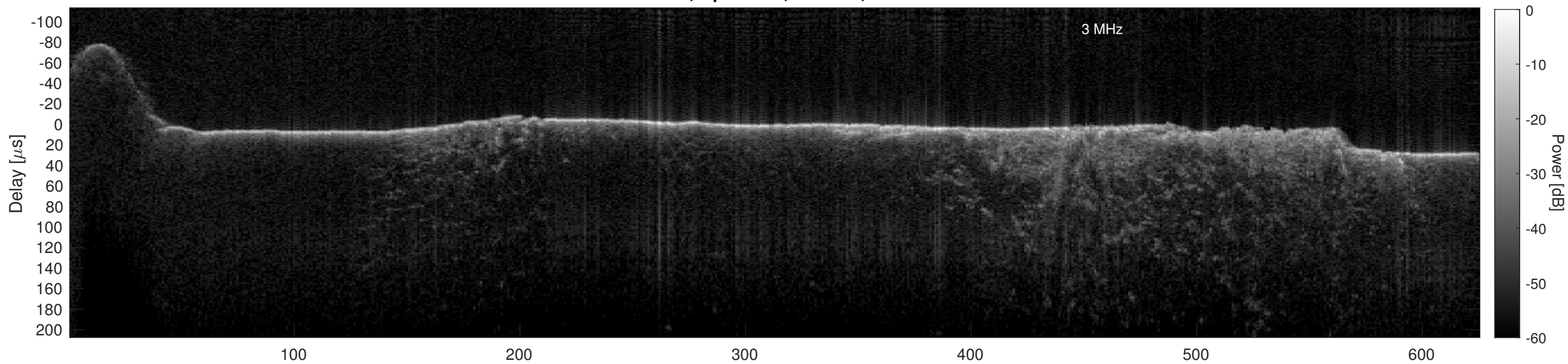
Orbit 21609, Cluttergram
