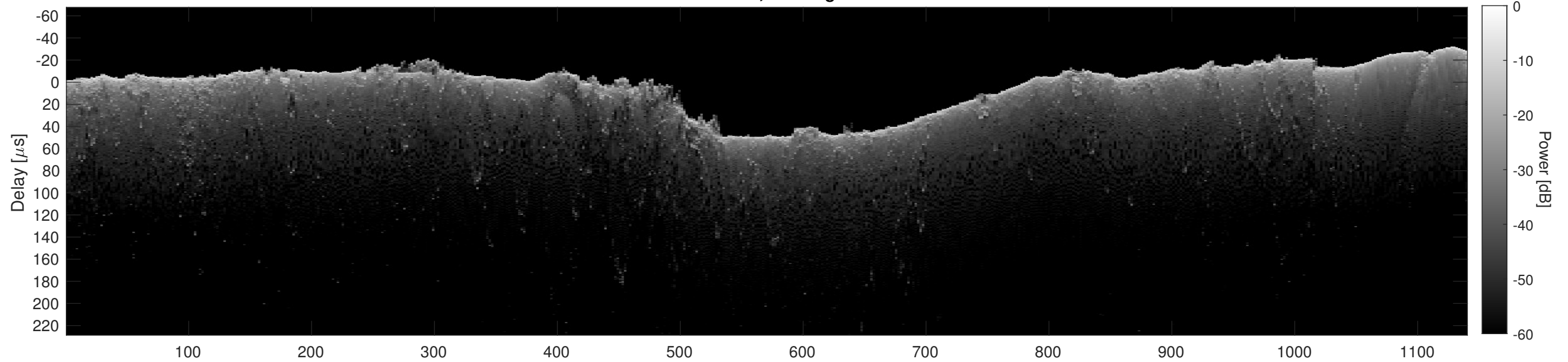
Orbit 21611, Cluttergram
