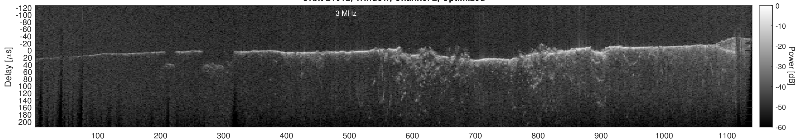
Orbit 21612, Cluttergram
