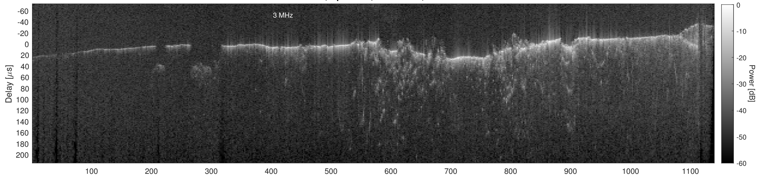
Orbit 21612, Cluttergram
