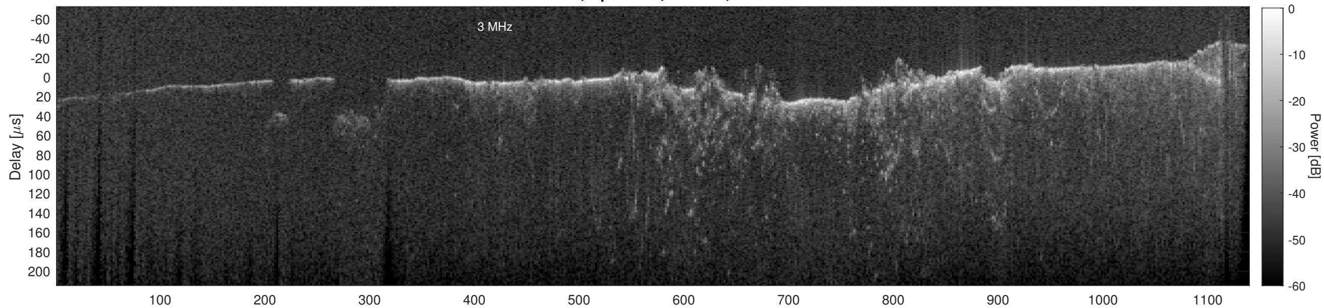
Orbit 21612, Cluttergram
