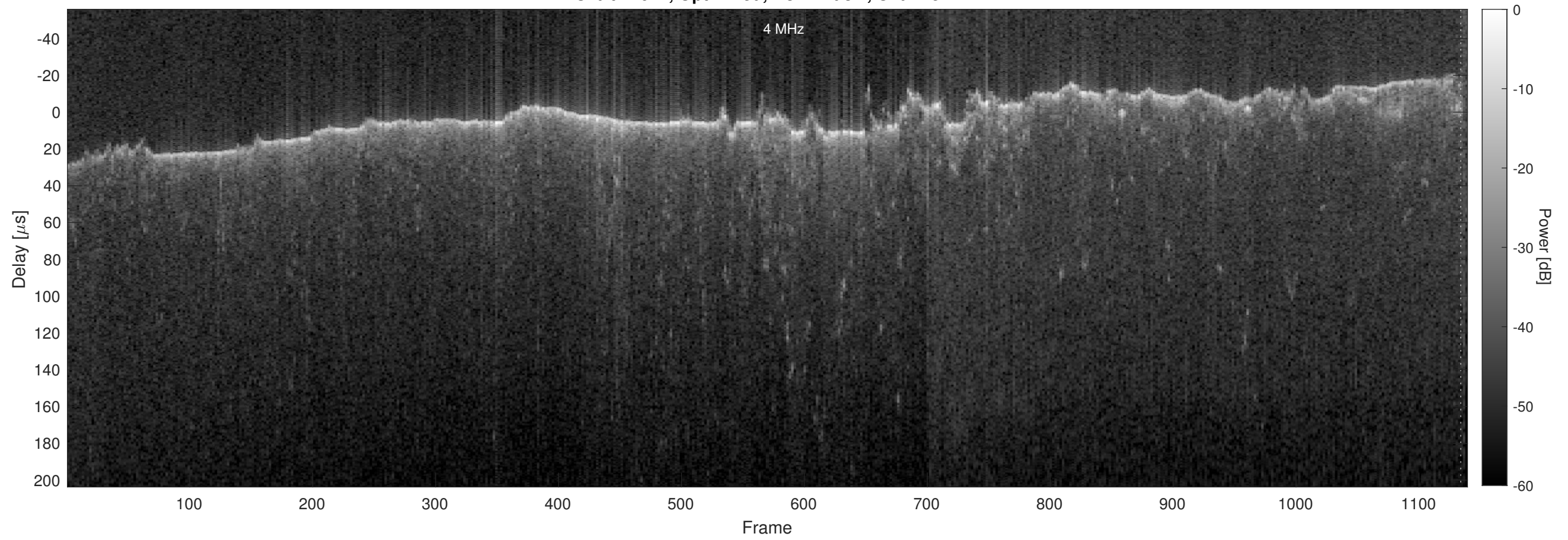
Orbit 21614, Optimized, No Window, Channel 2
