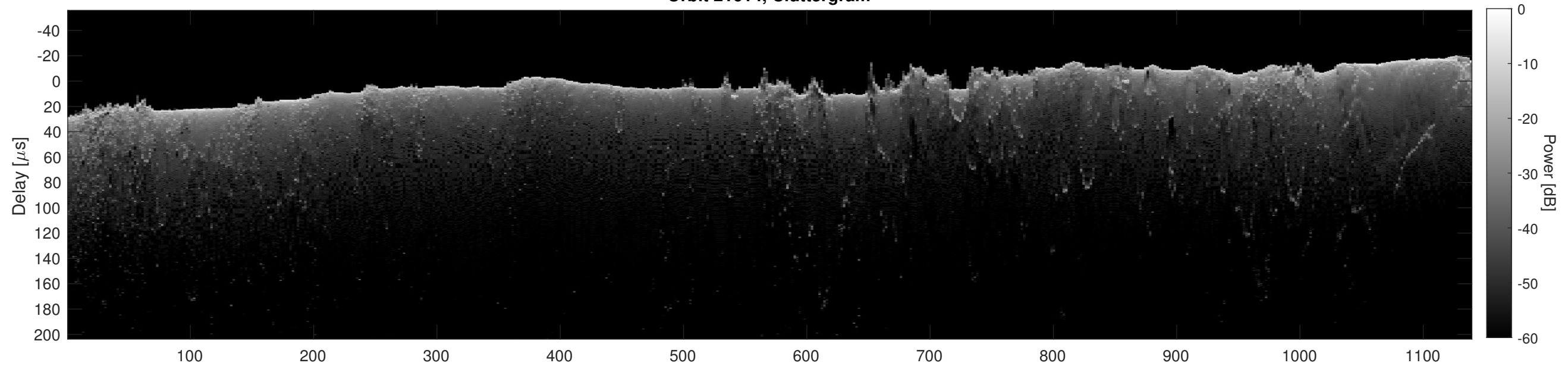
Orbit 21614, Cluttergram
